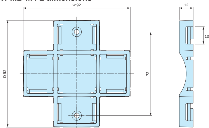
WPMB-M4-2 dimensions
