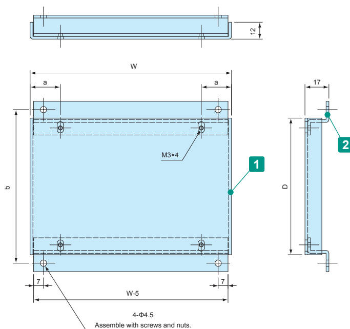
Assembly drawings
