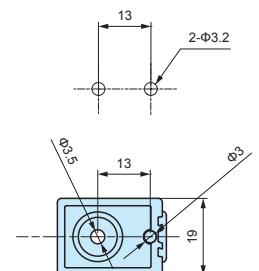
Mounting hole (Rear)
