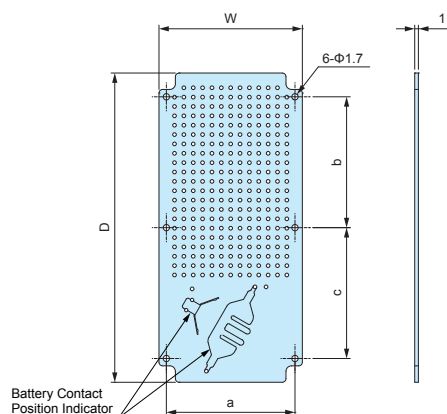
Battery Contact Position Indicator on CSPB-115
