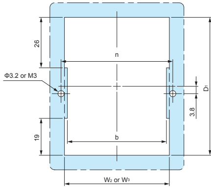
Mounting hole dimension
