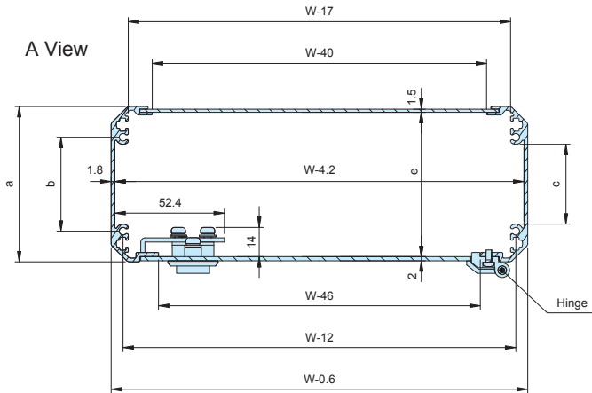
W Cross-section
