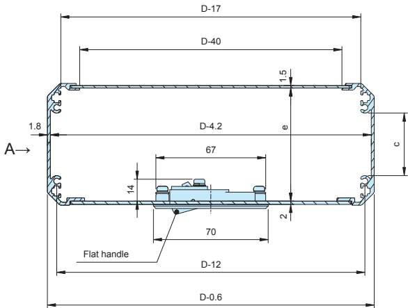
D cross-section
