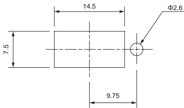
Hole layout for installing
