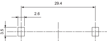
PCB layout top view
