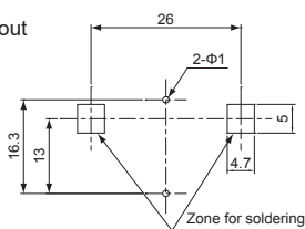
BK-888 + BK-2032M PCB layout top view
