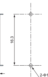
Installation hole layout
