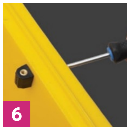
6 Tighten the screw firmly. (Recommended torque : 0.8 ~ 1.0 N · m)
