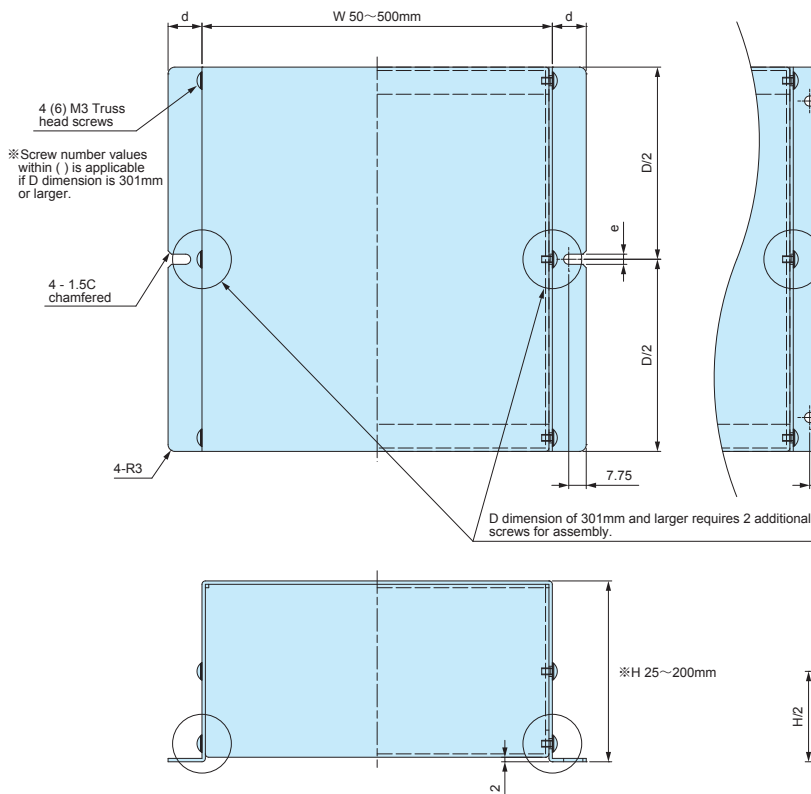
2-hole flange type
