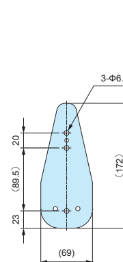
Wall mounting bracket dimensions
