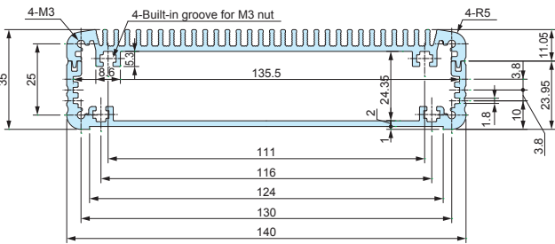
EXHS141-36-□
