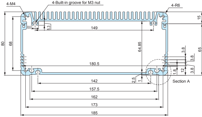
EXHS187-82-□
