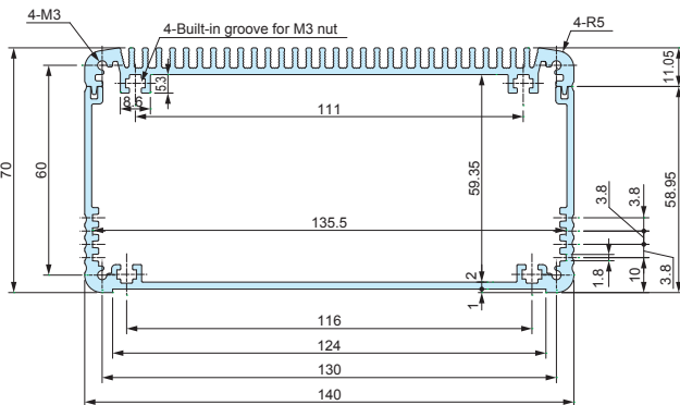
EXHS141-71-□
