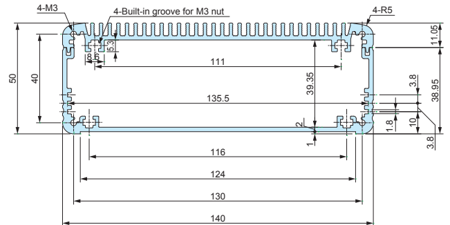
EXHS141-91-□
