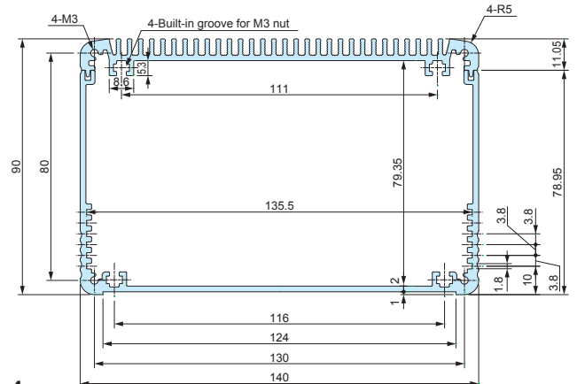
EXHS141-91-□
