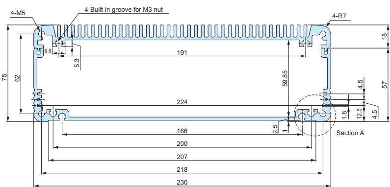
EXHS232-77-□
