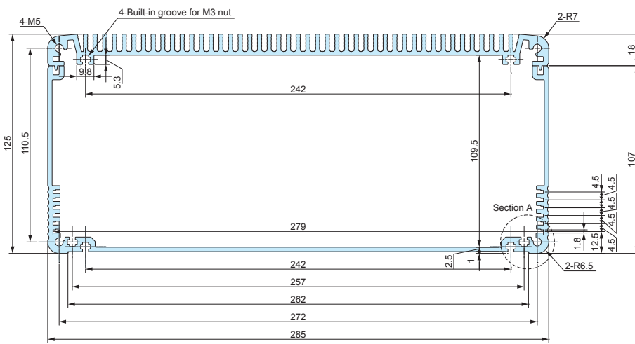
EXHS288-128-□
