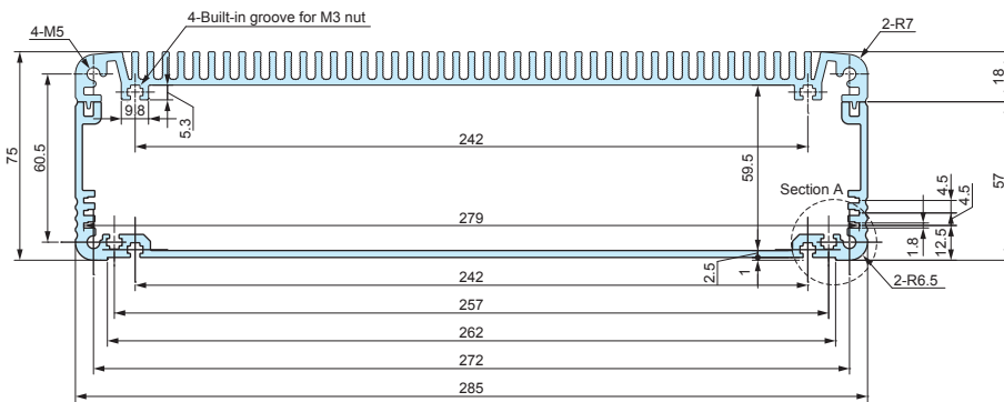
EXHS288-78-□
