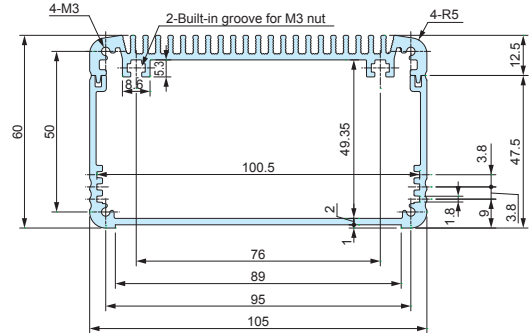
EXHS141-51-□
