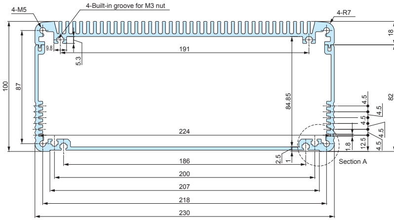
EXHS232-102-□
