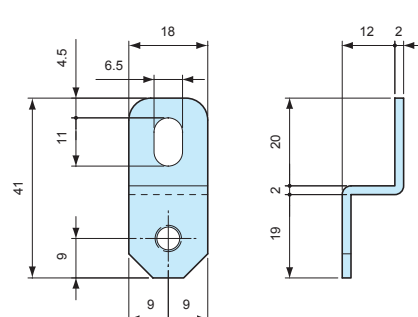
CK-26P dimensions
