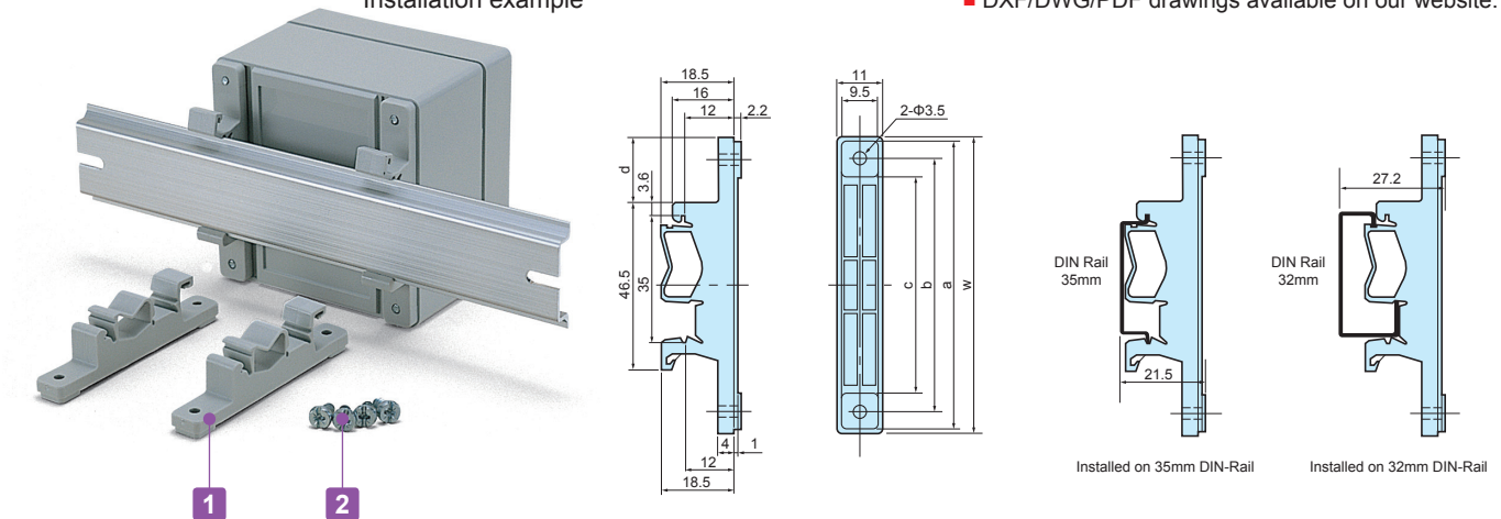
Installation example
