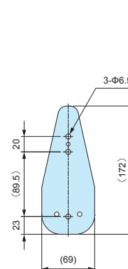
Wall mounting bracket dimensions
