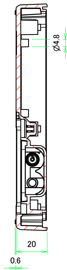
B-B (1:1.5)
