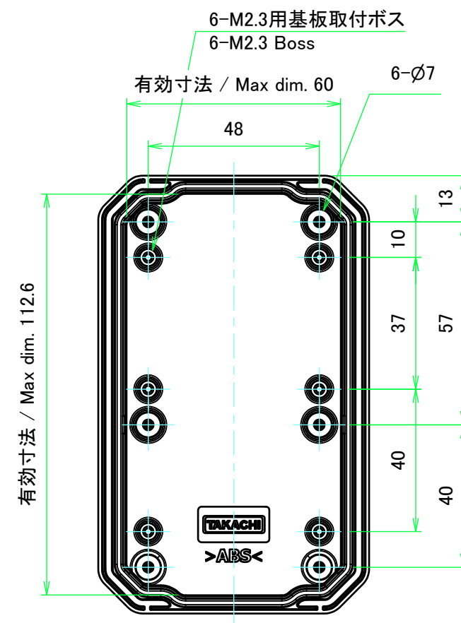
B-B (1:1.5)
