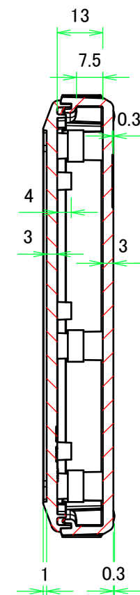
B-B (1:1.5)
