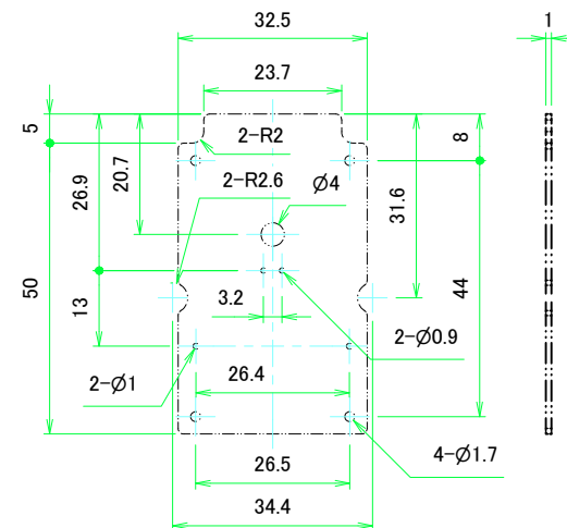
推奨基板形状 / Recommended PCB dimension
