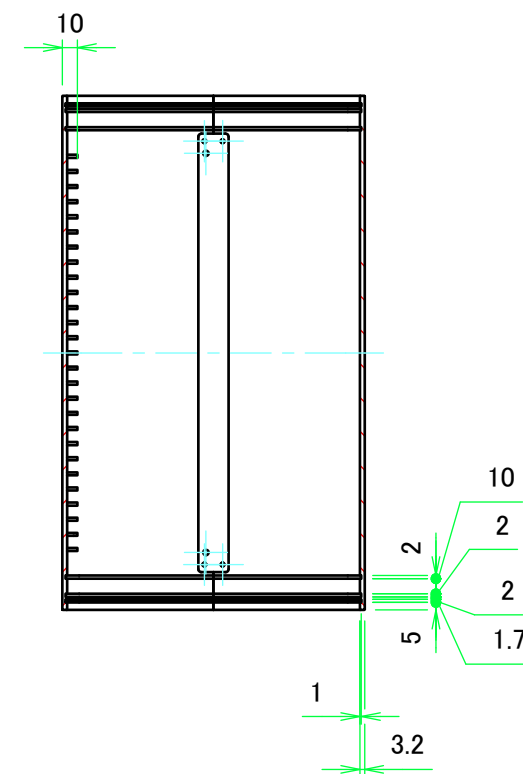
B-B (1:5)
