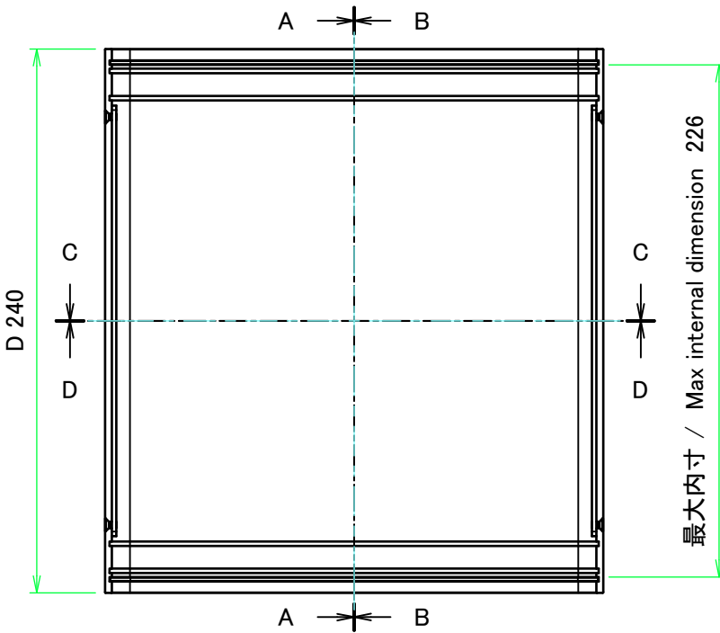
下カバー(内視) Bottom cover (Internal view)
