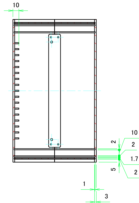
B-B (1:3)
