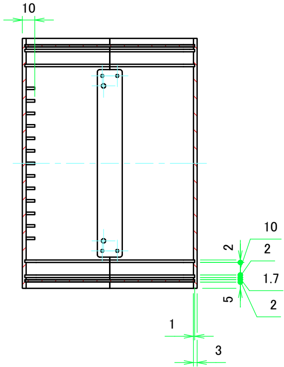
B-B (1:3)
