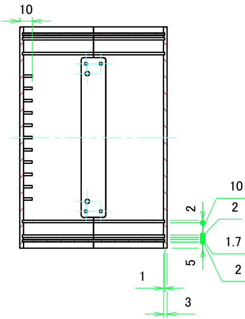
B-B (1:3)
