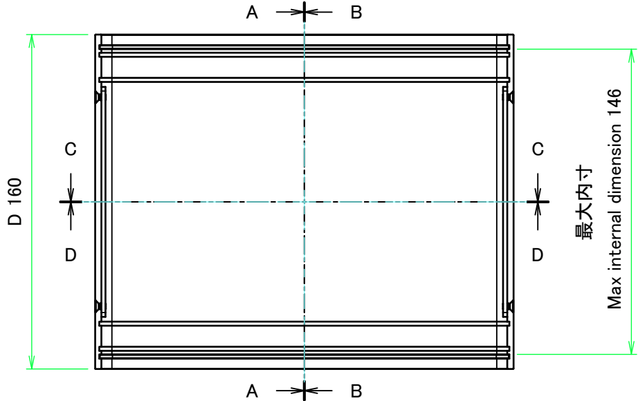
下カバー(内視) Bottom cover (Internal view)
