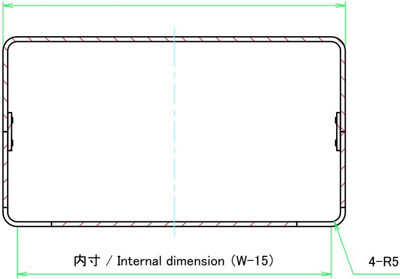
下カバー(内視) Bottom cover (Internal view)
