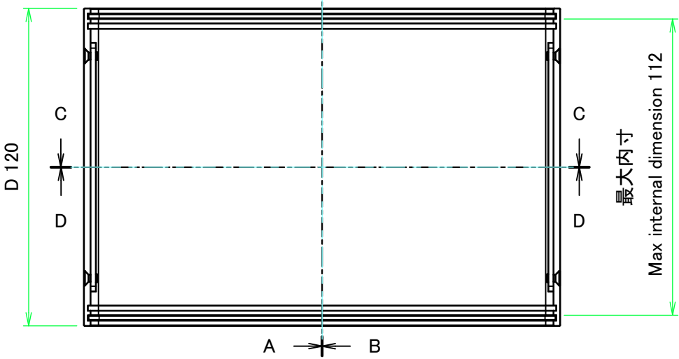
下カバー(内視) Bottom cover (Internal view)
