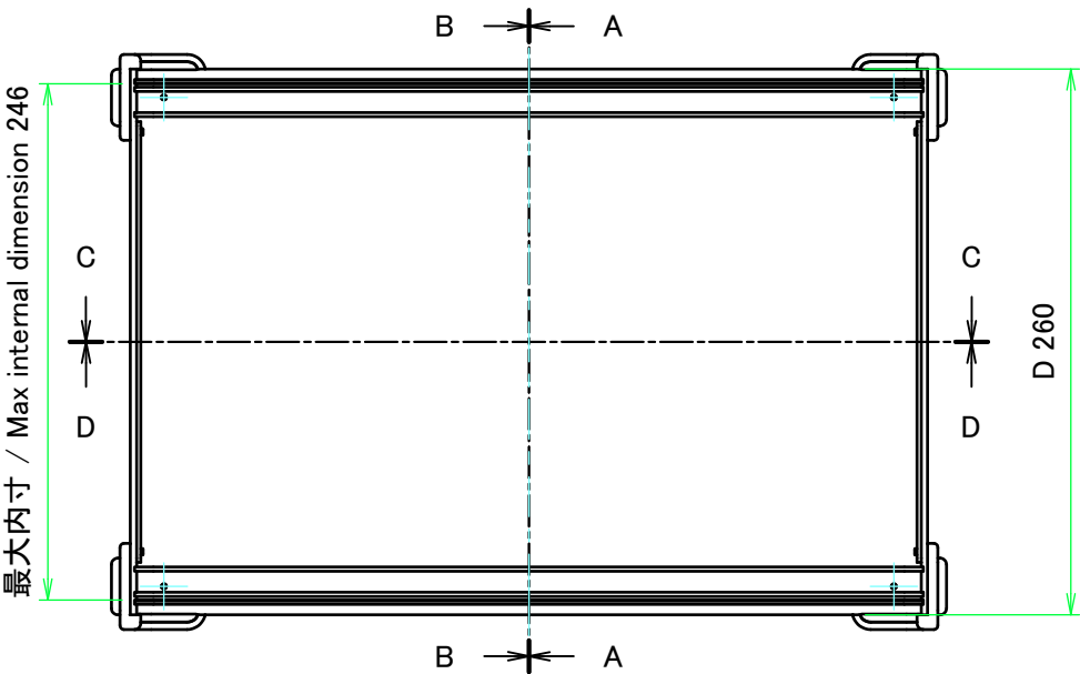
下カバー(内視) Bottom cover (Internal View)
