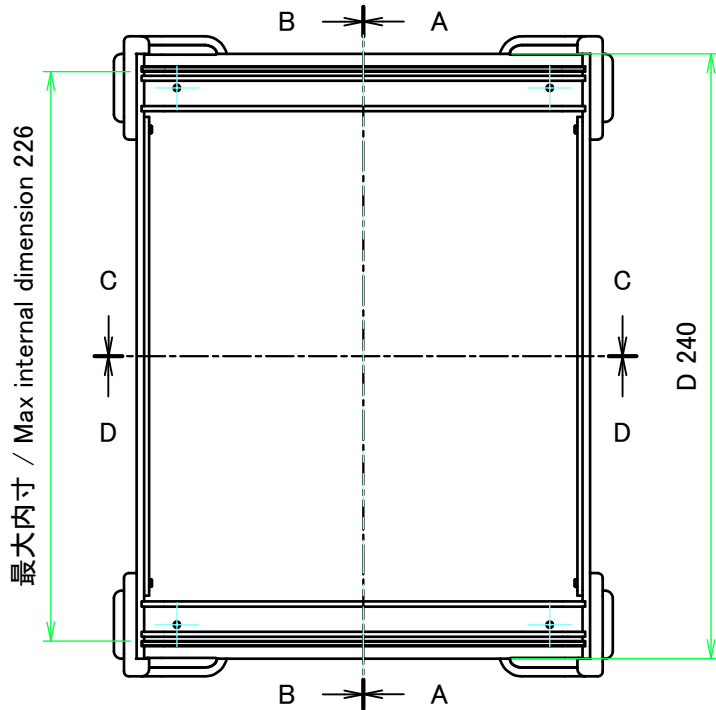
下カバー(内視) Bottom cover (Internal View)
