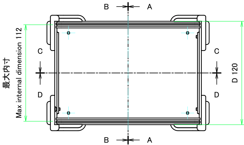
下カバー(内視) Bottom cover (Internal View)
