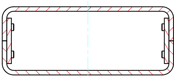
C-C (1:1)
