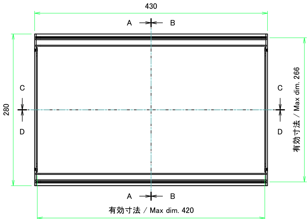
下カバー(内視) Bottom cover (Internal view)
