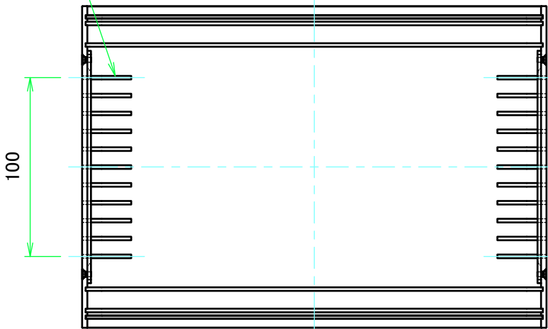
放熱穴 ( 2x30 P10 ) Ventilation slits ( 2x30 P10 )
