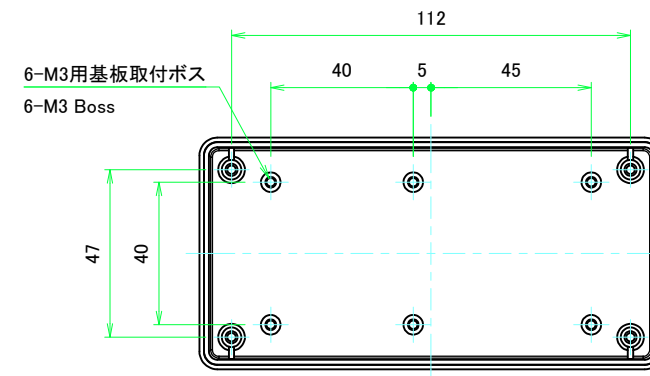
C-C (1:1.5)
