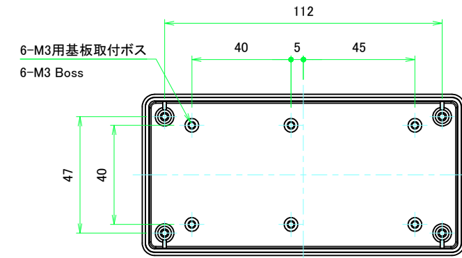
C-C (1:1.5)
