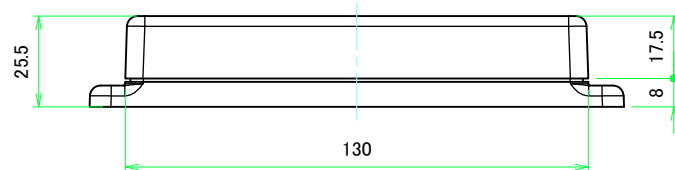
B-B (1:1.5)
