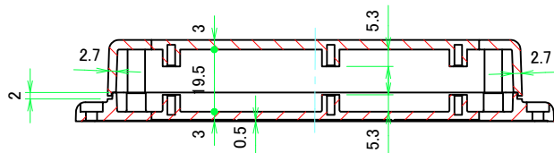
B-B (1:1.5)
