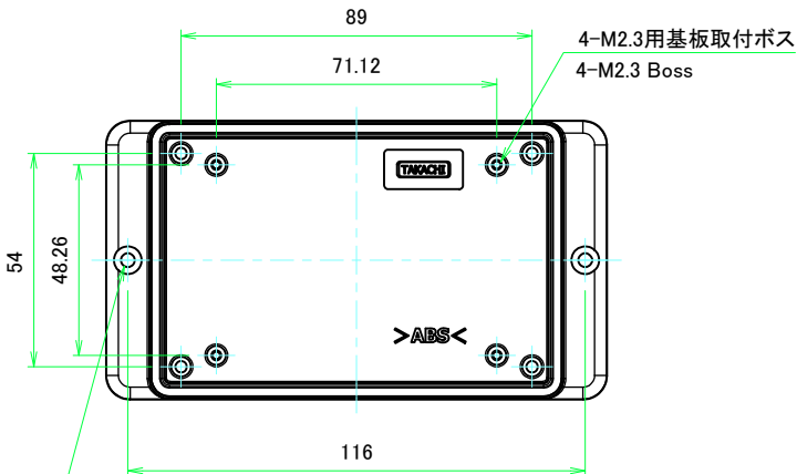
2-M3用壁取付穴 2-M3 Wall mounting hole
