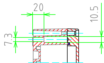
外部取付用穴 Extemal mount holes
