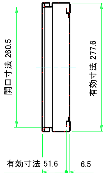
B-B (1:5)
