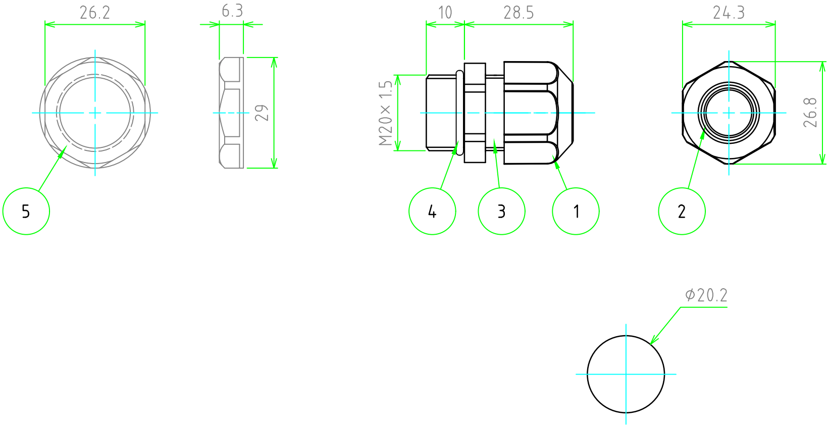
取付穴寸法/Mounting hole dimensions
