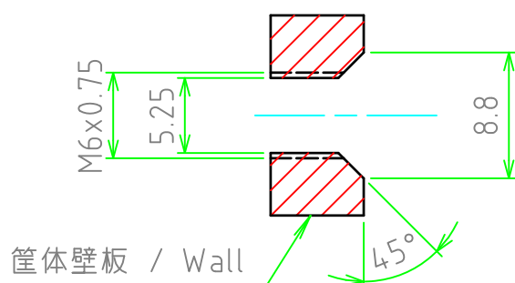
推奨穴加工図 / Recommended hole shapes for installing
