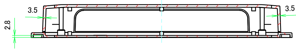
B-B (1:3)
