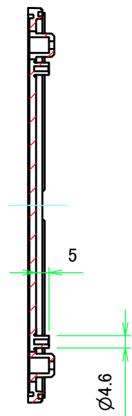
E-E (1:2)
