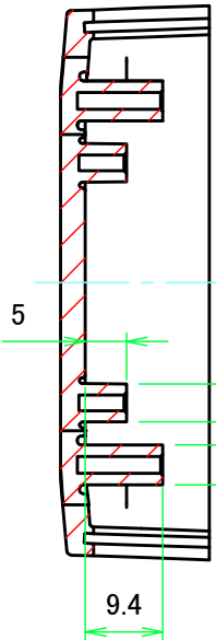
C-C (1:1)
