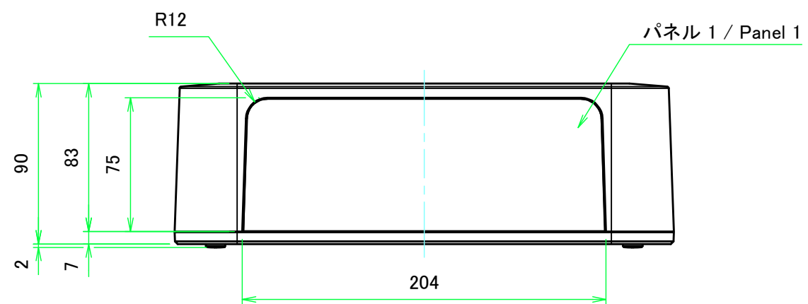
B-B (1:3)
