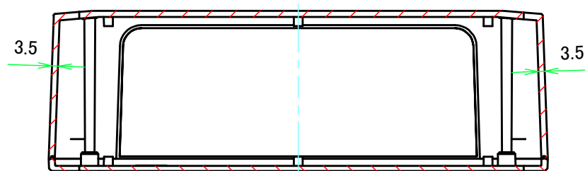
B-B (1:3)
