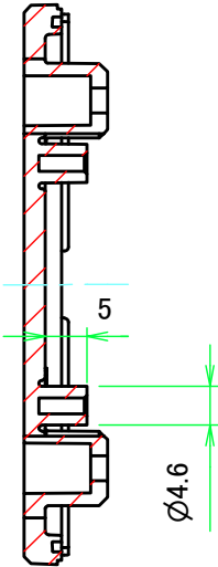
E-E (1:1)
