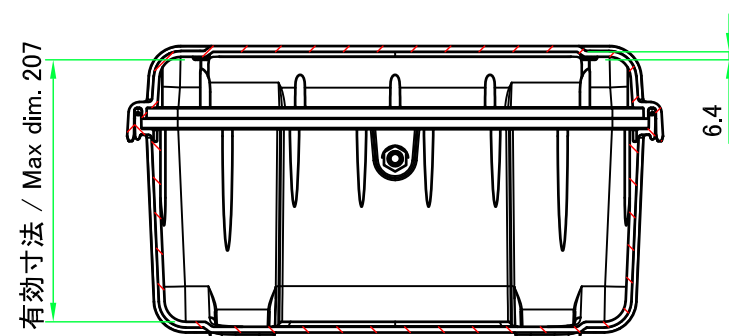
B-B (1:6)
