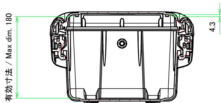
B-B (1:5)
