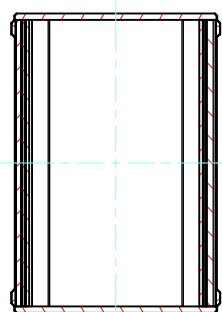
C-C (1:2.5)
