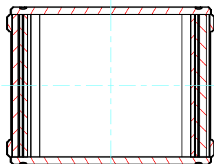
C-C (1:1.5)
