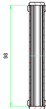
B-B (1:1.5)
