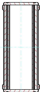
C-C (1:1.5)
