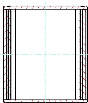
C-C (1:1.5)
