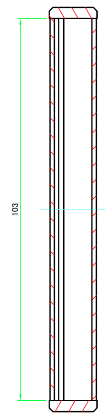
B-B (1:1)
